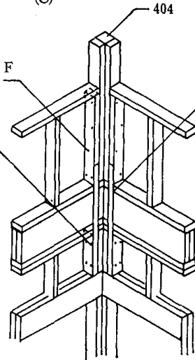
(C) 2階入隅部の緊結の詳細
